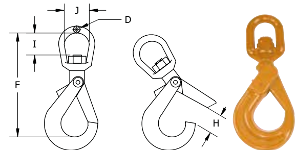
Stamped with BM identification code, size, grade and traceability code. Meet ASTM-952 standard.
