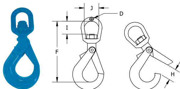
Stamped with BM identification code, size, grade and traceability code. Meet ASTM-952 standard.
