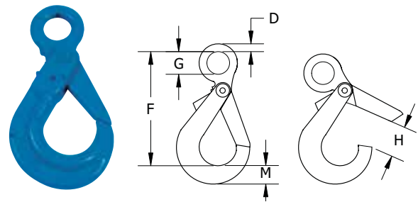
Stamped with BM identification code, size, grade and traceability code. Meet ASTM-952 standard.
