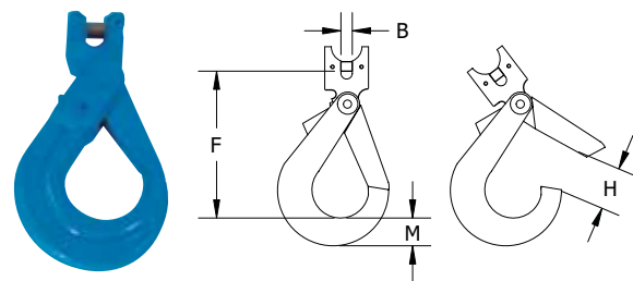
Stamped with BM identification code, size, grade and traceability code. Meet ASTM-952 standard.
