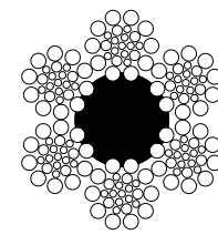
6 x 26 Fiber core
