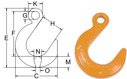
Stamped with BM identification code, size, grade and traceability code. Meet ASTM-952 standard.
