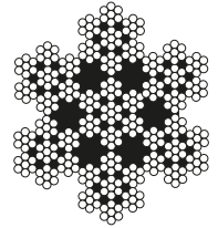
7 x 7 x 7
