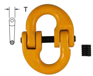
Stamped with BM identification code, size, grade and traceability code. Meet ASTM-952 standard.
