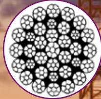
35 x 7 (compacted)
