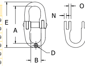
Stamped with BM identification code, size, grade and traceability code. Meet ASTM-952 standard.
