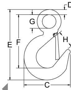
Stamped with BM identification code, size, grade and traceability code. Meet ASTM-952 standard.
